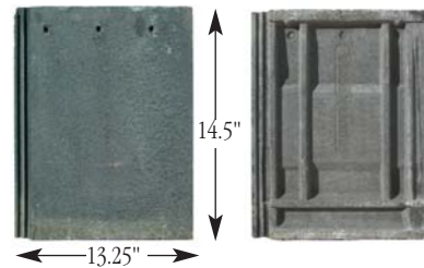
Marley Country Slate Flat shingle style concrete tile from Celotex
