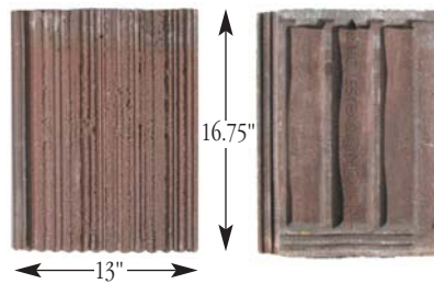
Homestead Shake Flat shake style, textured concrete tile from Monier.
