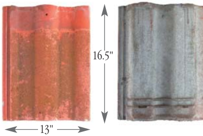
Roma Small Barrel Small barrel-style concrete tile manufactured by Monier.
